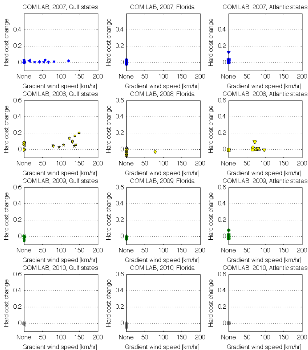
Figure B.11: Observed hard cost change from July to January versus wind speed by U.S. region and year (2007–2010) for the commercial labor component basket.
